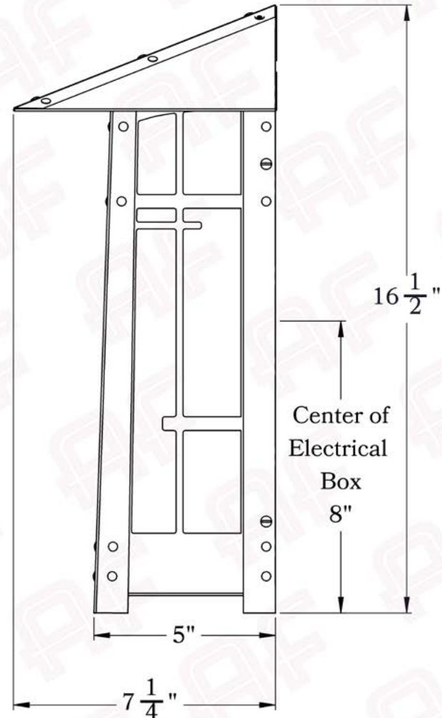
SIDE VIEW
